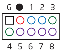
Fig. 4 Receiver connections
