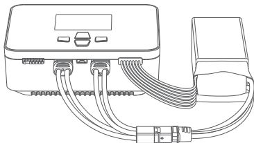
Paralled charge
